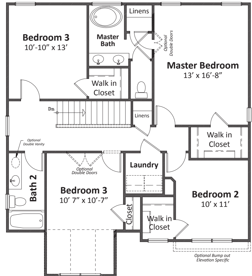
2 nd Floor
